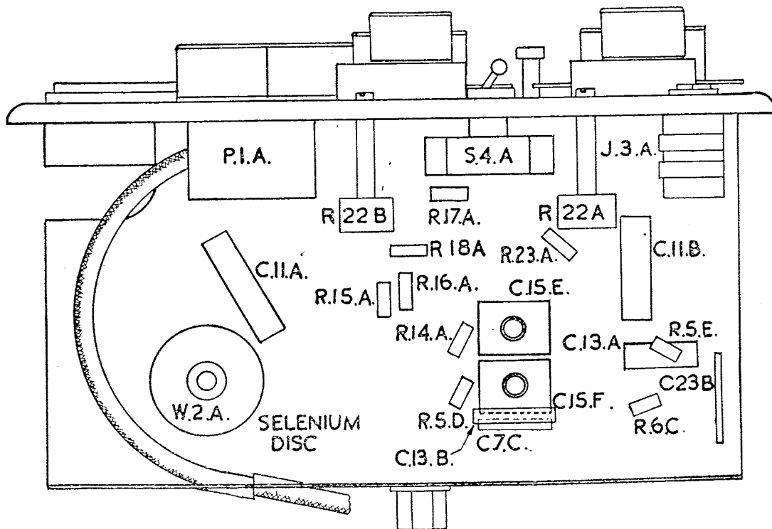
FIG. 6. UNDERSIDE VIEW OF CHASSIS
