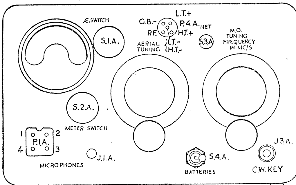
FIG. 7. FRONT VIEW OF RECEIVER PANEL
