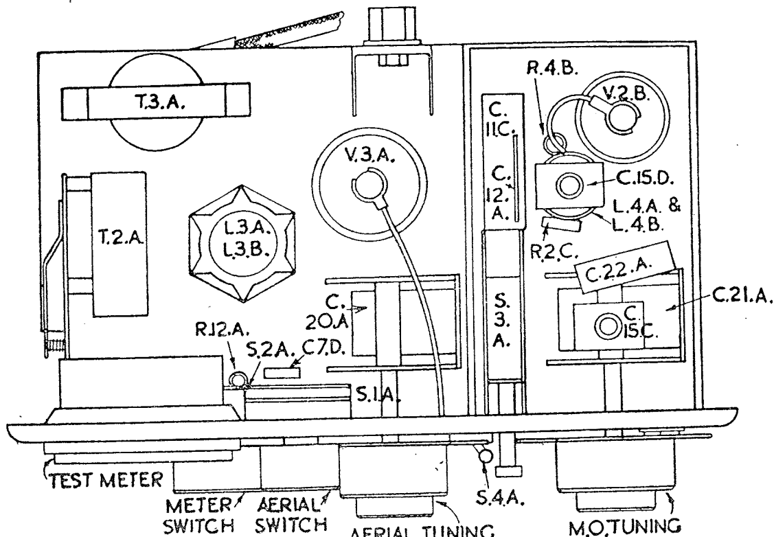
FIG. 5. TOP VIEW OF CHASSIS
