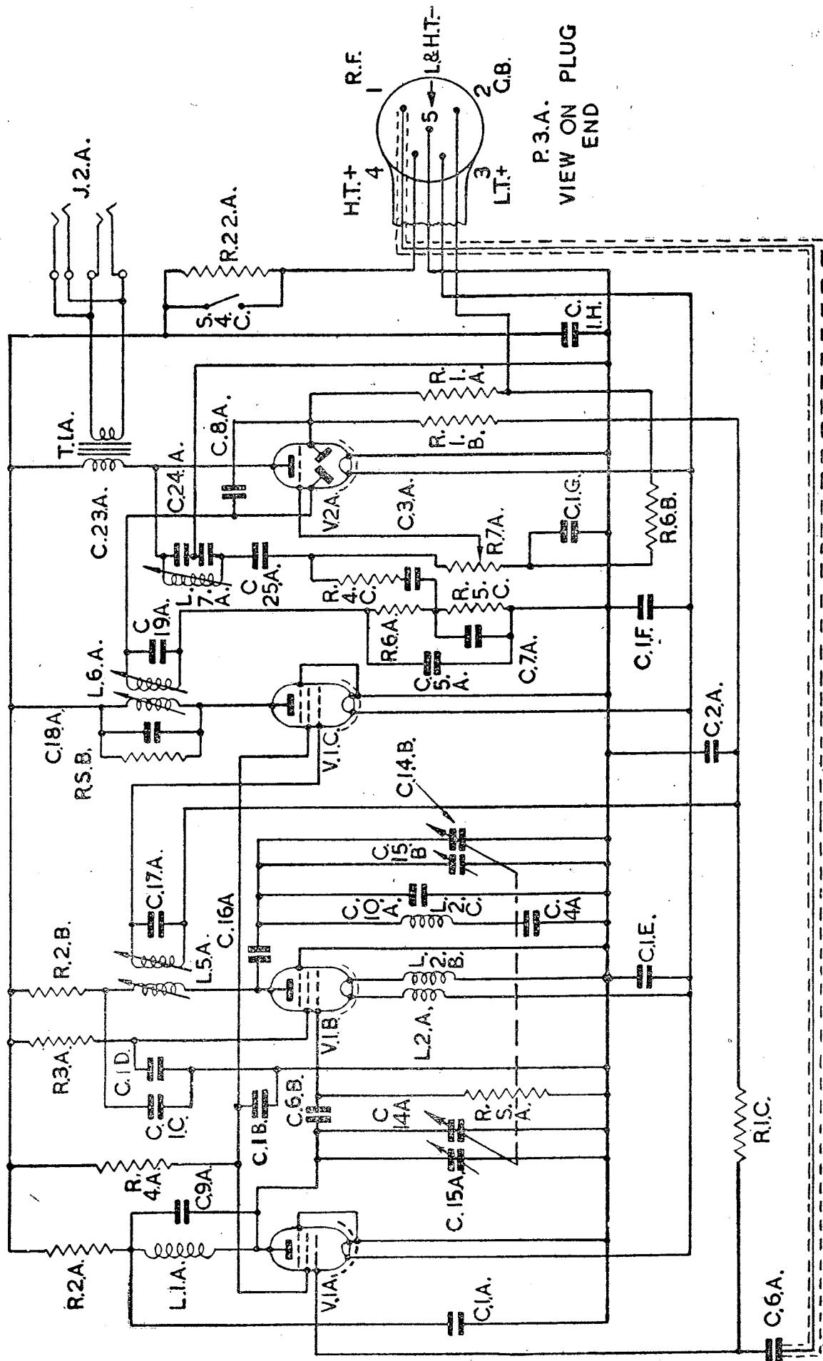
WIRELESS-SET No. 18 MARK III RECEIVER FIG. 14
