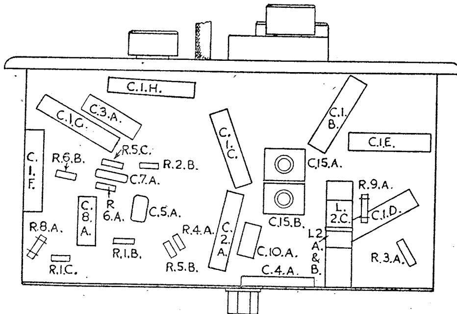
FIG. 10. UNDERSIDE VIEW OF CHASSIS
