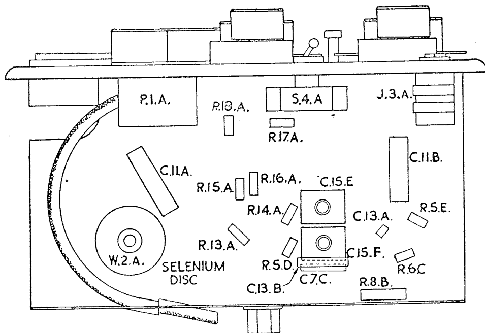
FIG. 12. UNDERSIDE VIEW OF CHASSIS
