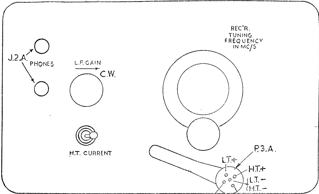
FIG. 1. FRONT VIEW OF RECEIVER PANEL
