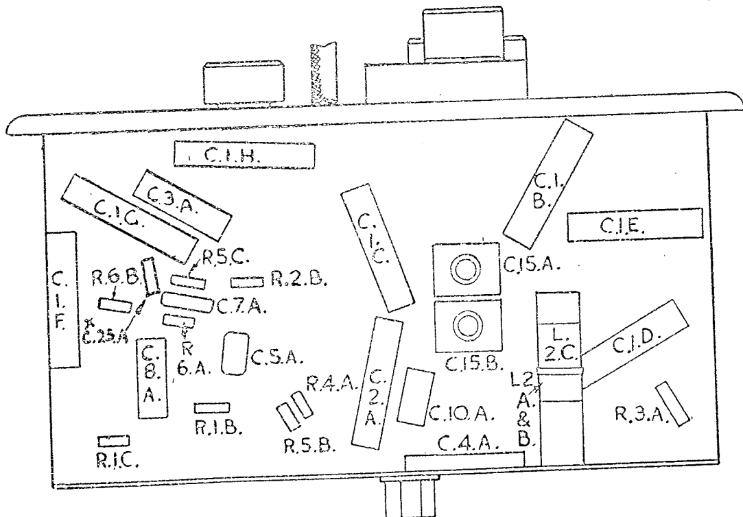
FIG. 4. UNDERSIDE VIEW OF CHASSIS
