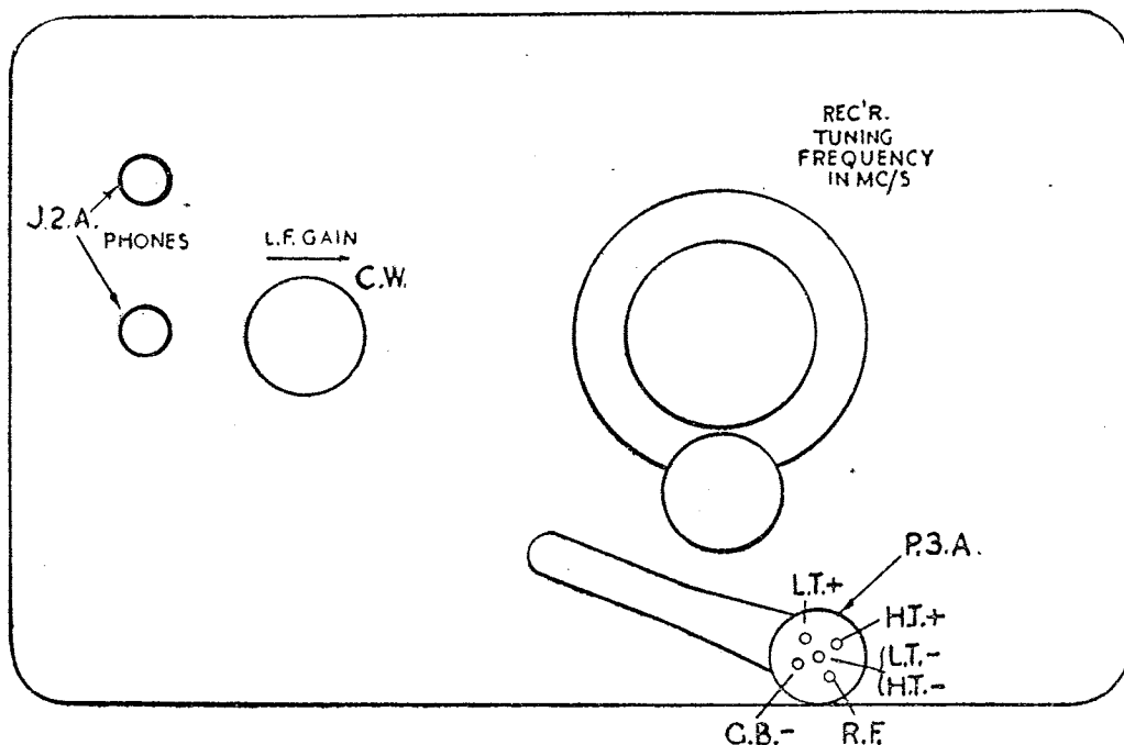
FIG. 7. FRONT VIEW OF RECEIVER PANEL
