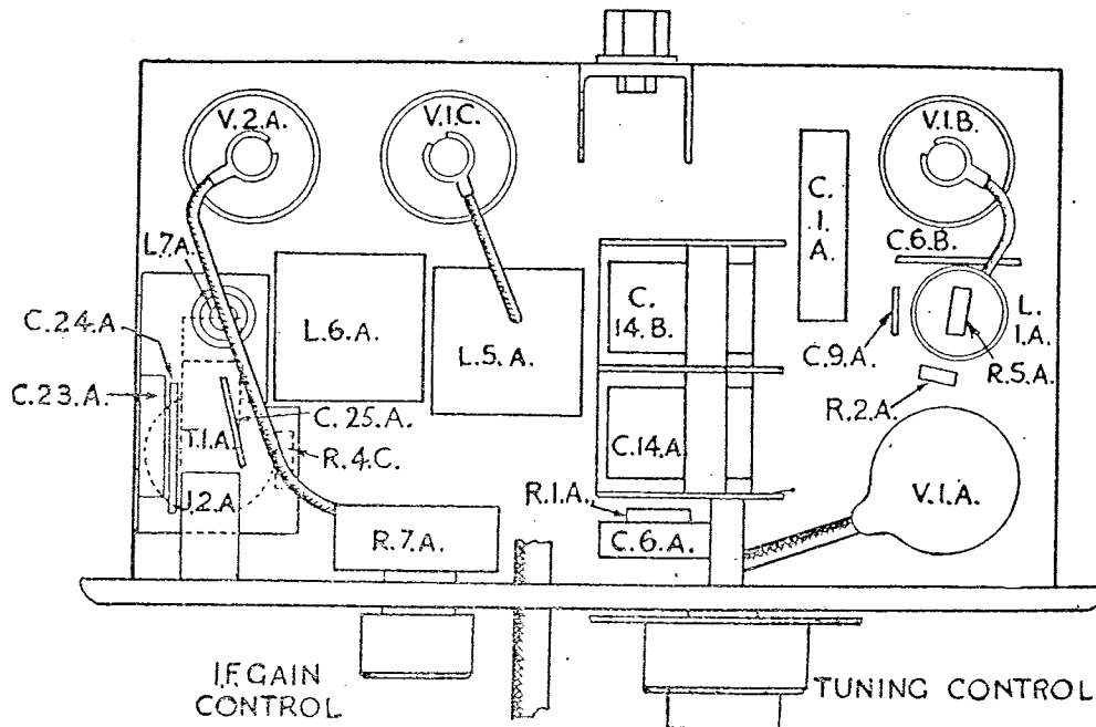
FIG. 9. TOP VIEW OF CHASSIS
