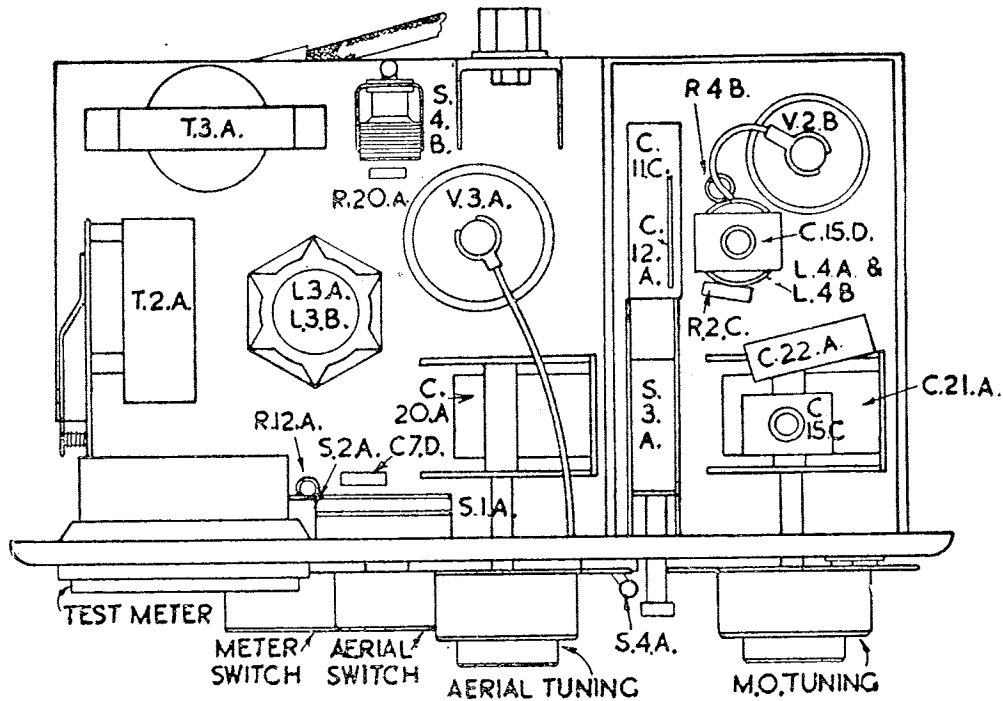
FIG. 11. TOP VIEW OF CHASSIS
