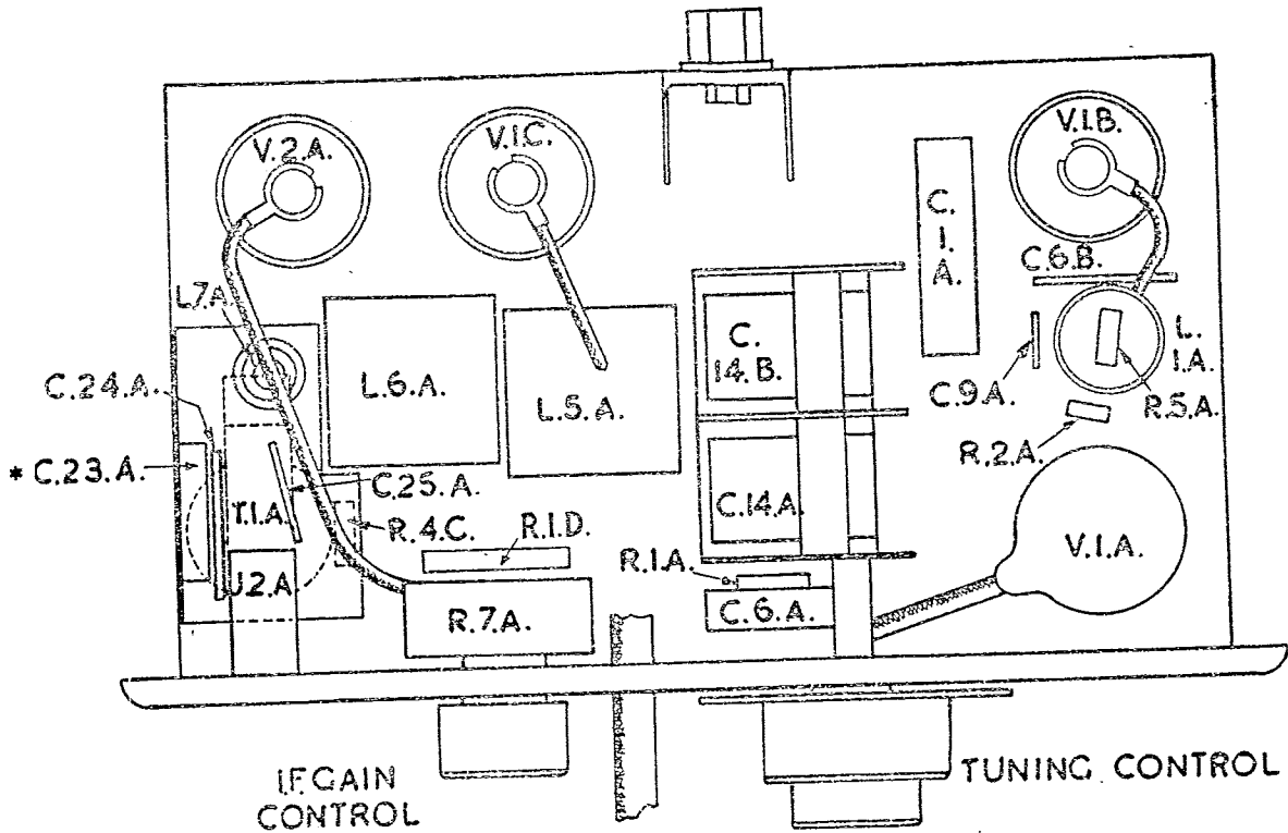
FIG. 3. TOP VIEW OF CHASSIS
